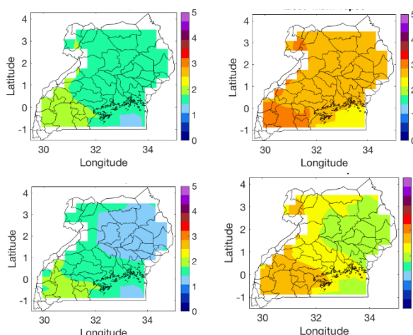
Figure 2. Projected seasonal mean changes in temperature for 2030s (LEFT) and 2050s (RIGHT) under the RCP8.5 emission scenario (worst case scenario), relative to the reference period (1961-2005). NOTE: In the 2050s, temperature in the potato growing areas is likely to rise by about 2.8°C - 3.0°C and 2.0°C - 2.8°C in the first (MAM; TOP RIGHT) and second (OND; BOTTOM RIGHT) season, respectively.
